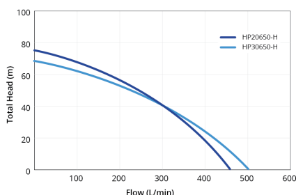
Performance Curve
